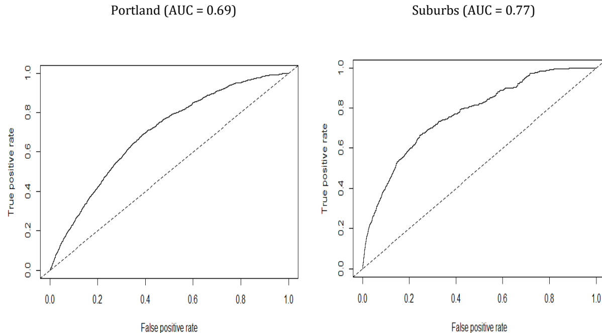
Figure 23: Area-Under-the-Curve Goodness of Fit Plots
