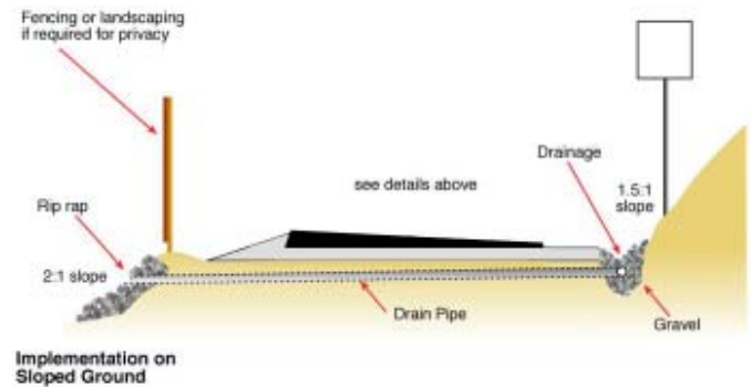
Typical Multi-Use Trail Section
