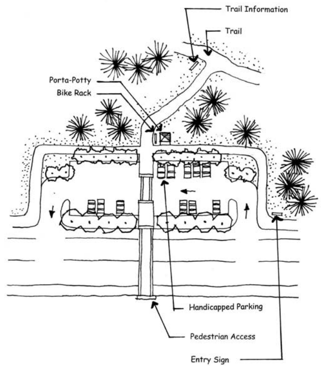
Potential Trailhead Design
